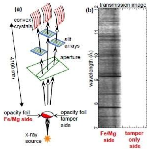
Figure 5: Experiment. a: spectrometers view the “half-moon” shaped tampered iron/magnesium sample. Each spectrometer employs multiple slits to project space-resolved images onto a convex crystal that disperses the spectrum before recording on film. The setup measures the unattenuated (tamper only) and the attenuated (tamper plus FeMg) spectra on the same experiment. b: A space and spectrally-resolved transmission image is obtained by dividing the attenuated spectral image by the unattenuated image. Darker regions correspond to higher absorption. The white portion of the image corresponds to 100% transmission [1] .
