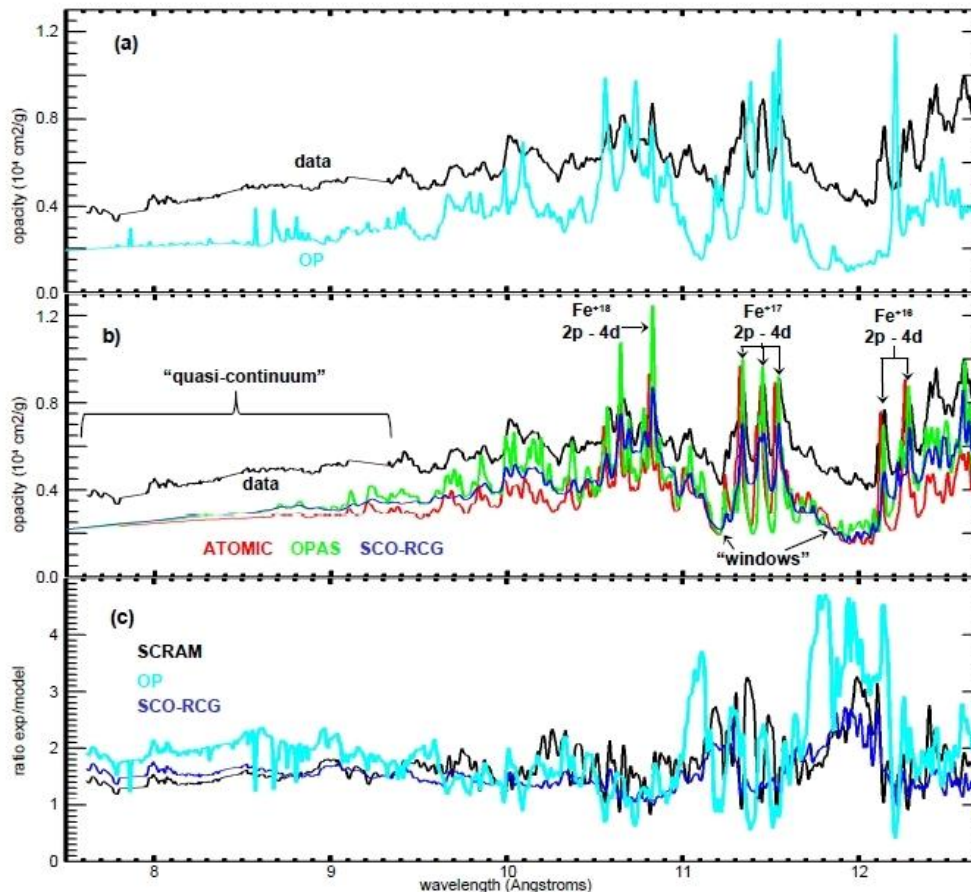
Figure 7: Comparisons of observed iron opacity spectra (black curve) with multiple models. OP (cyan, at top and bottom panels), SCO-RCG (blue), ATOMIC (red), OPAS (light green) at the solar convection zone boundary temperature and density: T_e = 2.11 MK, n_e = 3.1 \times 10^{22} cm -3 . a. OP model uses for solar modeling. The dashed lines are the Rosseland mean opacities calculated for this wavelength range. b. Comparisons with three other models. c. Ratio of the experiment opacity with three different models [1]. Considerable differences can be seen between the measured and predicted opacities
