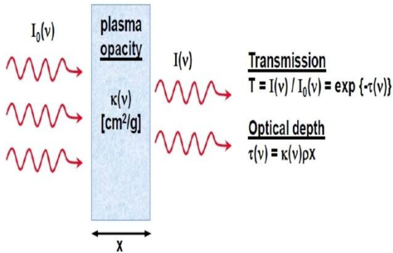
Figure 2: Change in intensity of radiation passing through a distance of "x" in the plasma is due to the opacity.
