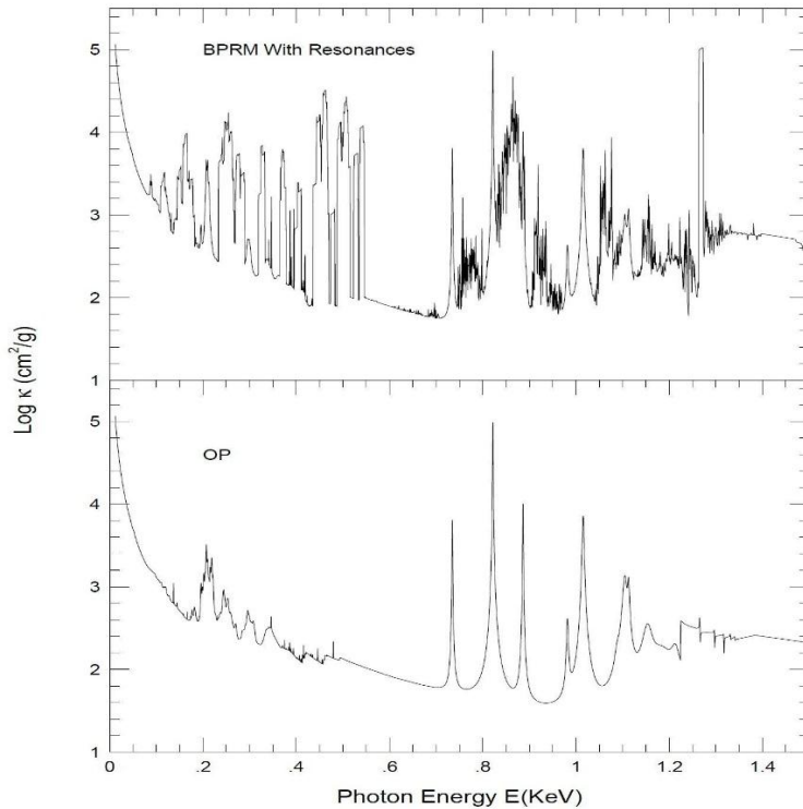
Figure 8: Monochromatic opacity of Fe XVII at temperature T = 2.24 \times 10^6 K and electron density N_e = 10^{23} \text{ cm}^{-3} , corresponding to the base of the solar convection zone. The top panel presents opacity obtained using new atomic data from 60 CC wave function expansion and the bottom panel the total OP opacities which uses TOPbase data [14]. OP model includes resonances of high core-excitations, which are not included in the wave function expansion, as lines which are broadened with autoionization widths perturbatively, and the high-energy K-shell continuum opacity not yet included in 60-CC calculations [8]
