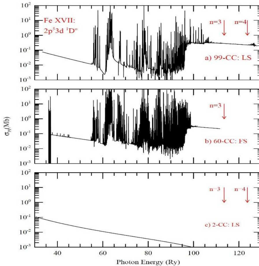
Figure 9: Photoionization cross sections \sigma_{pI} of 2s^22p^53d(^1D^o) state of Fe XVII in the R-matrix calculations: a) present 99-CC expansion in LS coupling, b) 60-CC expansion in fine structure (FS) [8], c) 2-CC expansion in LS coupling under the OP [14]. The arrows indicate energy positions for the last n=3 and n=4 core excitations. \sigma_{pI} in FS (b) has more resonances due to couplings of more channels and finer energy mesh and in 99-CC LS (c) has additional resonances, although not very strong, and a very slow decaying background.
