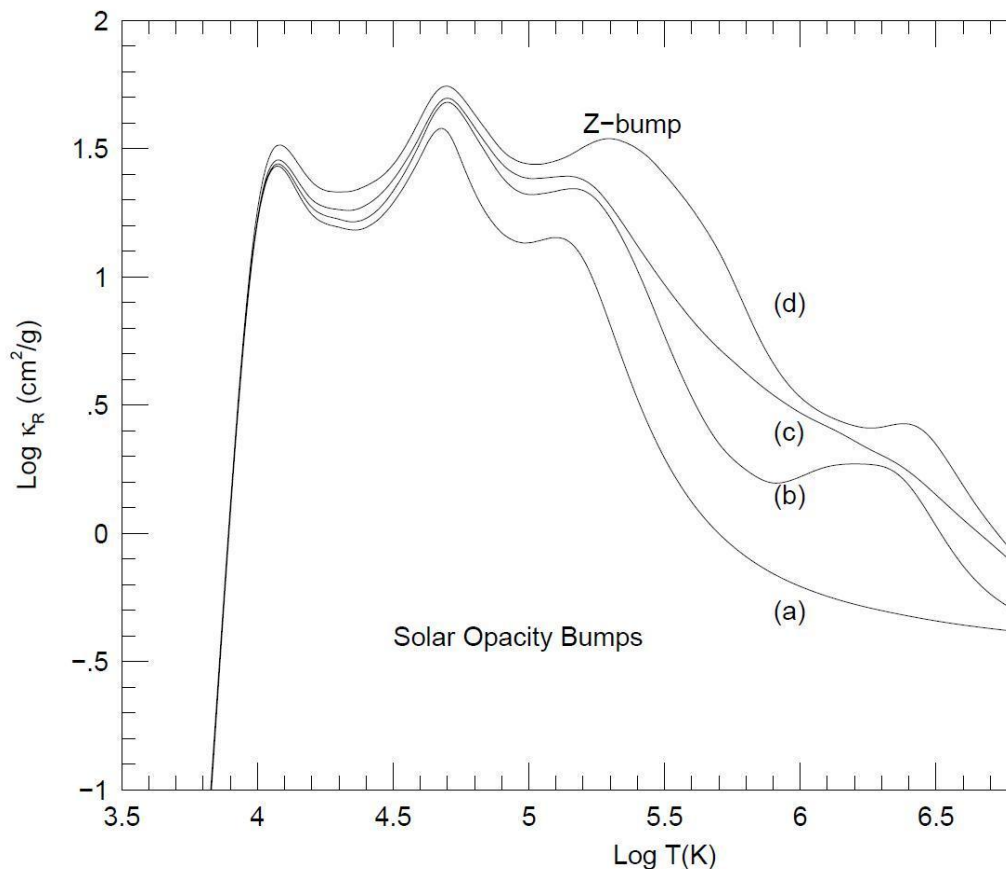
Figure 3: Increment of Rosseland mean opacity \kappa_R with elements at R=-3 . R = \rho(g/cc)/T_6^3 , T_6 = T * 10^{-6} is related to depths in a star. Several bumps associated with excitation and or ionization of different atomic species are seen. The first (lowest \kappa_R ) curve (a) has three bumps corresponding to the ionization of neutral H, He, and He II, at Log T \approx 4, 4.6, and 5.2 respectively. Including elements up to Ne raises the opacity towards higher temperatures as in curve (b). In addition, another bump appears at Log T \approx 6 - 6.5 which is related to highly ionized ions. Addition of further elements up to Ca raises the overall opacity significantly as shown in curve (c). The topmost curve (d) is due to the further inclusion of the iron group elements up to Ni, that gives rise to a considerable increase in opacity for all T > 10^4 K. The most outstanding enhancement in opacity due to iron occurs curve (d), Log T = 5.2 - 5.6 , referred to as the Z-bump. It is mainly due to excitation and ionization of Fe ions with partially filled M-shell ( n = 3 ), Fe IX -Fe XVI [16] .
