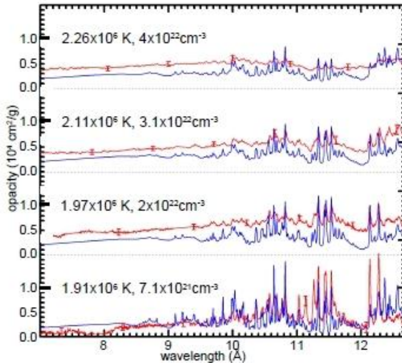
Figure 6: Measured iron opacity spectra (red) at four T_e/n_e values are compared with predicted values (blue) calculated using the SCRAM model which accounts for the instrument resolution. With higher temperature and density the measured opacity becomes more featureless while the background shows larger difference with the predictions [1] .
